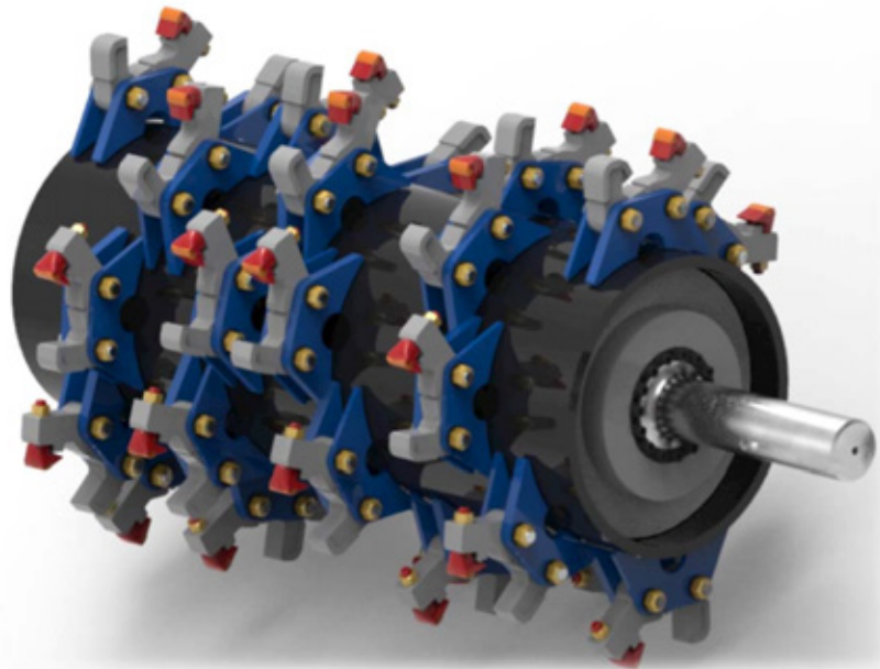
Standard 30-tooth mill 2680XP and 3680XP
